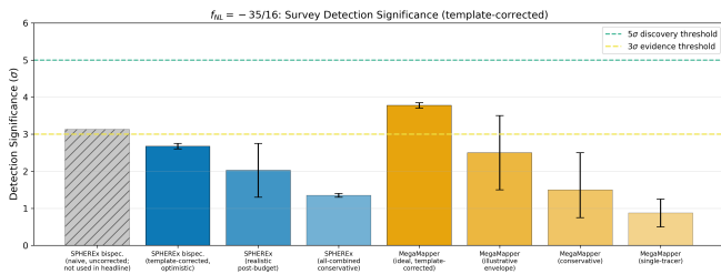
FIG. 2. Detection significance for the corrected central f_{\text{NL}} = -35/16 across survey configurations. SPHEREx bars (left to right): naive uncorrected 3.13\sigma (reference only); template-corrected optimistic 2.6 – 2.75\sigma ( |f_{\text{NL}}| r/\sigma , noise-weighted r = 0.84 ); realistic post-systematic-budget envelope 1.3 – 2.75\sigma ; and all-combined conservative endpoint 1.3 – 1.4\sigma . MegaMapper bars: ideal 3.7 – 3.85\sigma ; 1.5 – 3.5\sigma design-uncertainty envelope; conservative; single-tracer. All values are exactly one-half of what the erroneous -35/8 input would give (details in Sec. VII).
