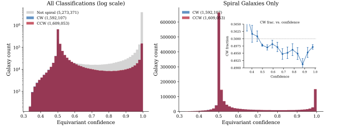
FIG. 6. Distribution of maximum-class confidence \max(P_{\text{CW}}, P_{\text{CCW}}, P_{\text{NS}}) for all 8,474,531 galaxies. Strongly bimodal: 73.6% at \max p \geq 0.9 (high-confidence labels) + a long tail of indeterminate cases ( \max p < 0.5 , dominated by NS/edge-on systems). The high-confidence (HC) cuts at p_{\text{eq}} > 0.6 ( N = 949,584 ) and p_{\text{eq}} > 0.8 ( N = 624,660 ) used in the systematics cross-checks (§E) are indicated.
