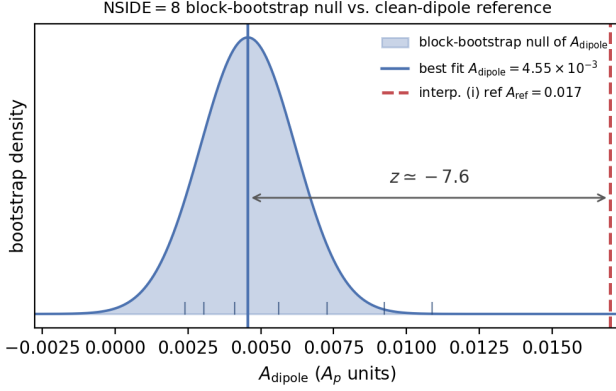
FIG. 10. Block-bootstrap sampling distribution of the FS-C dipole amplitude. NSIDE= 8 block-bootstrap resample distribution of A_{\text{dipole}} ( A_p units) from the joint 9-template WLS fit ( N_{\text{boot}} = 1000 , 440 in-mask superpixels, seed 42), rendered from the committed percentile array ( pipelines/p2_chirality/outputs/canonical_provenance/joint_nuisance_bootstrap_sigma.json ): best fit A_{\text{dipole}} = 4.55 \times 10^{-3} with spatial-coherence-inflated width \sigma_{\text{boot}} = 1.63 \times 10^{-3} ( 14.7\times the naive-WLS width). This is a block-bootstrap sampling distribution around the observed estimate, not a null distribution generated under A = A_{\text{ref}} . Blue band: block-bootstrap sampling distribution anchored on the committed mean/std; short vertical ticks mark the committed empirical \{0.5, 2.5, 16, 50, 84, 97.5, 99.5\} th percentiles of the resample distribution. Red dashed line: the interpretation-(i) clean-dipole reference amplitude A_{\text{ref}} = 0.017 (Shamir’s reported 1.7% asymmetry, already in A_p units). The reference sits z \simeq -7.6 from the fitted amplitude under the bootstrap covariance, i.e. a clean 1.7% cosmological dipole is disfavored; this is a template-model-disfavor statistic under the spatial error model, not a calibrated detection significance (see text).
