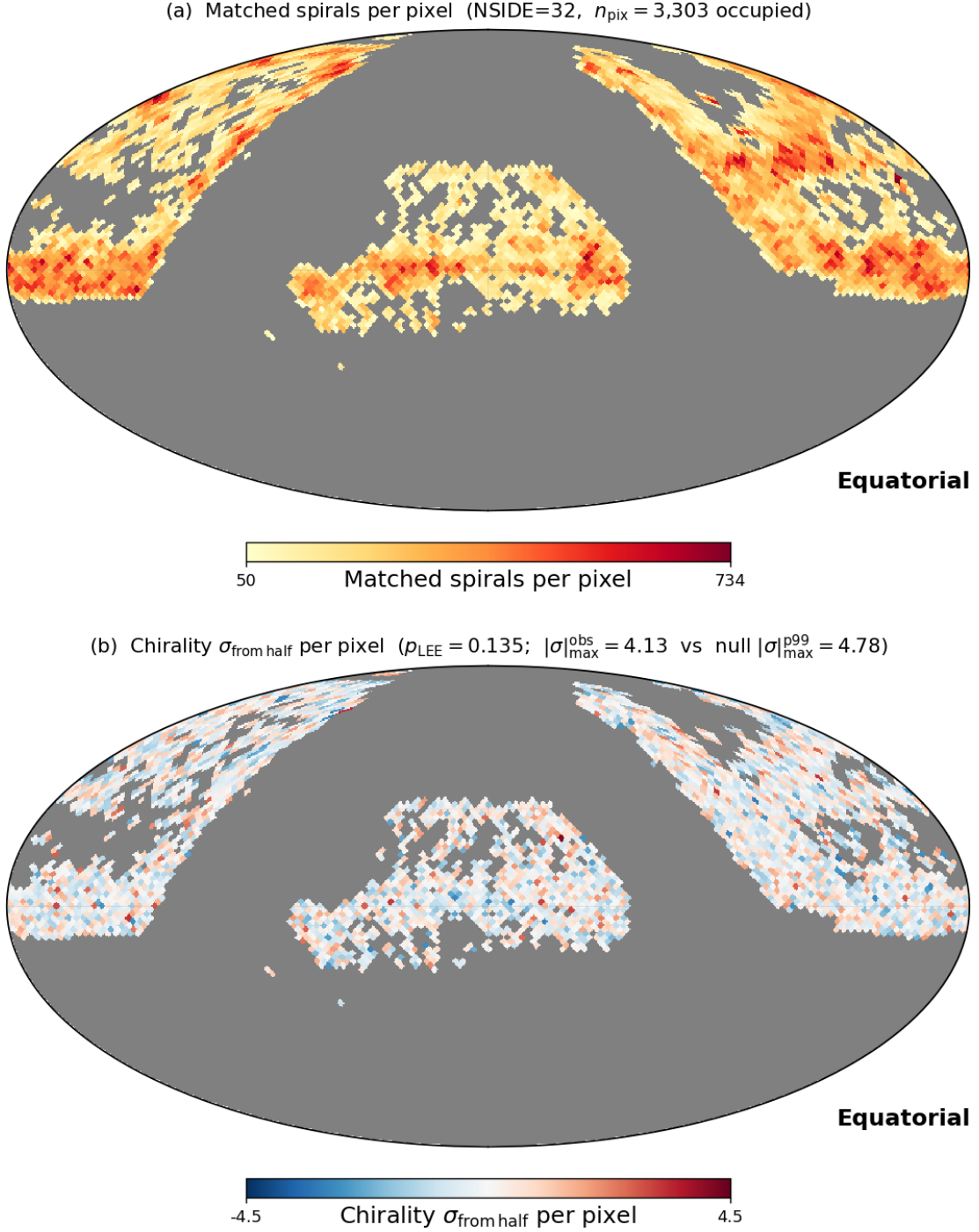
FIG. 6. NSIDE=32 Mollweide projections in equatorial coordinates. Top: matched-spiral count per occupied pixel. Bottom: per-pixel signed \sigma_{\text{from half}} for the chirality-relevant matched-spiral subsample. The observed |\sigma|_{\text{max}}^{\text{obs}} = 4.13 vs the label-shuffle null |\sigma|_{\text{max}}^{\text{null, p99}} = 4.78 gives a look-elsewhere p = 0.135 ; no NSIDE returns p < 0.05 . The map shows no coherent large-scale structure beyond random pixel-level scatter; the high- |\sigma| pixels are isolated rather than clustered, consistent with the counting-statistics distribution expected from label-shuffle.
