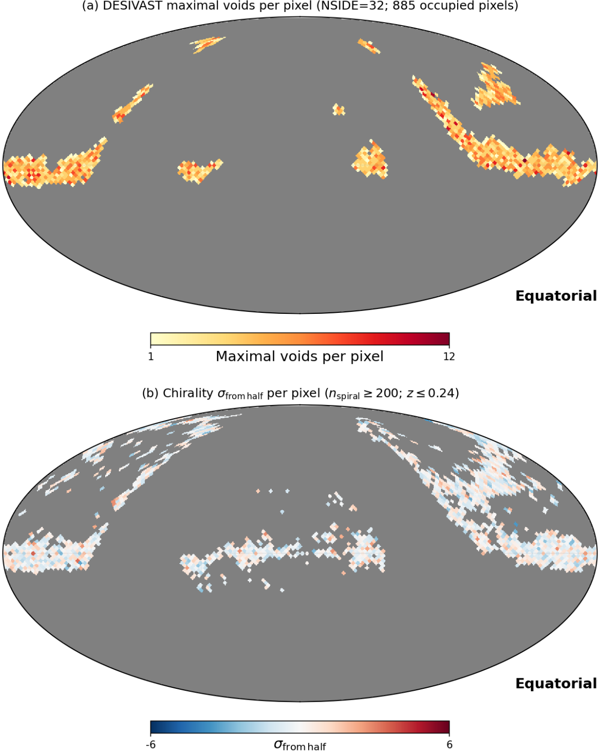
FIG. 8. HEALPix NSIDE = 32 Mollweide projection (equatorial coordinates). Top: count of DESIVAST maximal voids per pixel (885 occupied pixels at NSIDE = 32, median 4 voids/pix; the body text uses NSIDE = 16 for the sky-stratification table, yielding 297 occupied pixels at a coarser resolution). Bottom: per-pixel chirality \sigma_{\text{from half}} on the z \leq 0.24 matched-spiral subsample restricted to pixels with \geq 200 spirals (1,496 valid pixels, \sigma range -3.45 to +3.48 ). The Pearson correlation across the n_{\text{pix}}^{\text{both}} = 727 pixels containing both voids and \geq 200 spirals is r = 0.006 ( p = 0.88 ), statistically indistinguishable from zero.
