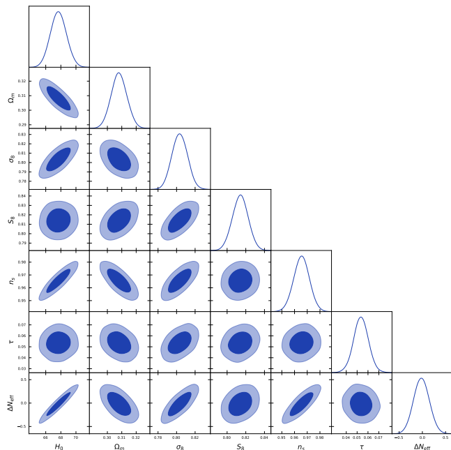
FIG. 8. Full-tension MCMC corner plot (119,617 post-burnin samples, getdist -thinned from 176,240 raw; footnote 9) over Planck+BAO+SN+H 0 +S 8 . The \Delta N_{\text{eff}} posterior is consistent with zero ( -0.020 \pm 0.169 ), confirming no additional relativistic species at recombination.
