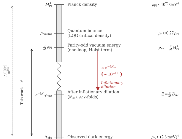
Energy density hierarchy: Planck scale \rightarrow observed \Lambda_{\text{obs}}
