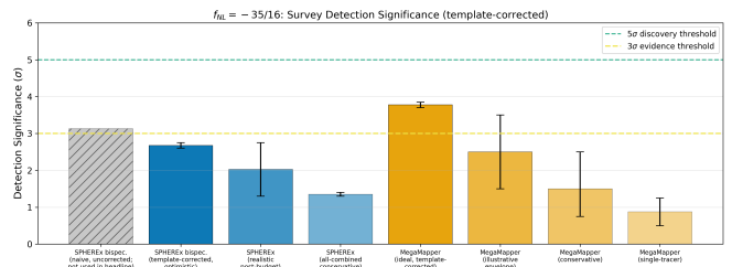
FIG. 2. Detection significance for the corrected central f_{\text{NL}} = -35/16 across survey configurations. SPHEREx bars (left to right): naive uncorrected 3.13\sigma (reference only); template-corrected optimistic 2.6 – 2.75\sigma ( |f_{\text{NL}}| r/\sigma , noise-weighted r = 0.84 ); realistic post-systematic-budget envelope 1.3 – 2.75\sigma ; and all-combined conservative endpoint 1.3 – 1.4\sigma . MegaMapper bars: ideal 3.7 – 3.85\sigma ; 1.5 – 3.5\sigma design-uncertainty envelope; conservative; single-tracer. All values are exactly one-half of what the erroneous -35/8 input would give (details in Sec. VII).
