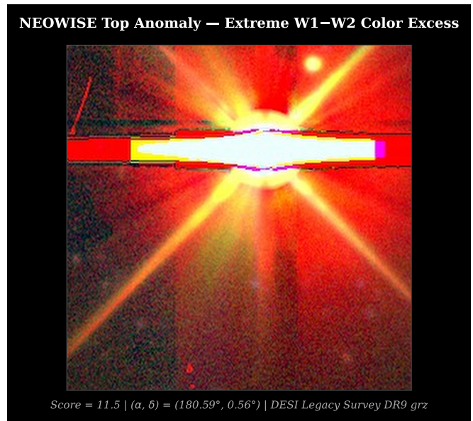
FIG. 5. NEOWISE top infrared anomaly at (\alpha, \delta) = (180.59^\circ, 0.56^\circ) , score = 11.5. DESI Legacy Survey DR9 grz composite, 256 \times 256 pixels at the native LS DR9 scale of 0.262"/px (256 \times 0.262" = 67" per side). Extreme W1–W2 infrared color excess; no prior SIMBAD entry within 5". The optical counterpart is a bright, saturated source with diffraction spikes indicative of a luminous red stellar or quasi-stellar object. Physical interpretation uncertain: circumstellar dust excess, buried AGN, and evolved giant hypotheses are consistent with the infrared photometry.
